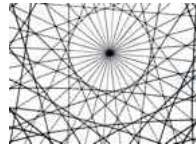
10 structure
